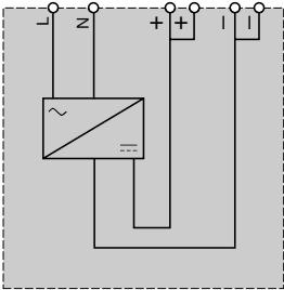
ABL 7RM power supply unit
