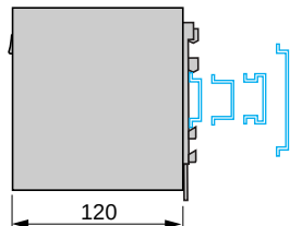
ABL-7RE24●●/ABL-7RP●●●● Common side view Mounting on 35 and 75 mm rails
