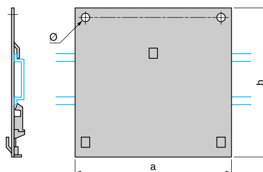
Mounting plates ABL-6AM0●
